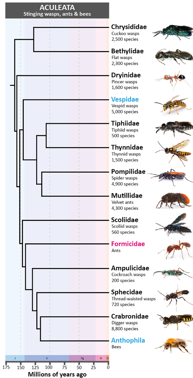
Fig. 1. Aculeate wasp diversity and their phylogenetic relationships. The aculeate wasps are a diverse, paraphyletic grouping of at least 33000 species across 22 families (Aguiar et al. , 2013; Branstetter et al. , 2017). For simplicity, this figure only includes 12 major aculeate wasp families (defined as those containing 200+ species); note that Formicidae and Anthophila are not aculeate wasps. Branch labels indicate the family name, common names (where available, taken from www.inaturalist.org ), and the approximate number of species within each family. Colour of branch labels indicates the levels of social organisation found within each taxon: black, all species are solitary; blue, family includes both solitary and social species; pink, all species are social. Phylogenetic relationships are simplified from Branstetter et al. (2017). Photograph credits (all under CC license or used with prior permission): Chrysididae – Owen (Figure legend continues on next column.)
